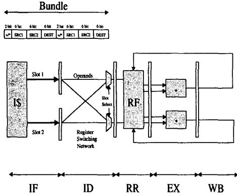
Figure 2: A simplified VLIW Pipelined Processor Architecture.
