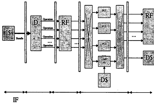
Figure 1: A general VLIW Pipelined Processor Architecture.
